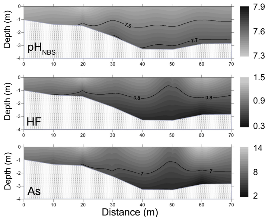
Fig. 3. Cross sections of: (a) seawater \text{pH}_{\text{NBS}} ; (b) the hydrothermal fluid (HF); (c) arsenic content (As) through the center of the study area in Fig. 1. The direction of the section from left to right is from the shore towards open water and parallel to and in between transects T2 and T3 in Fig. 1c.
